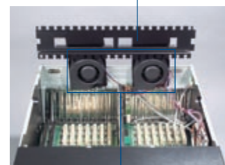
Hot-swap and easy-to-maintain cooling fan
